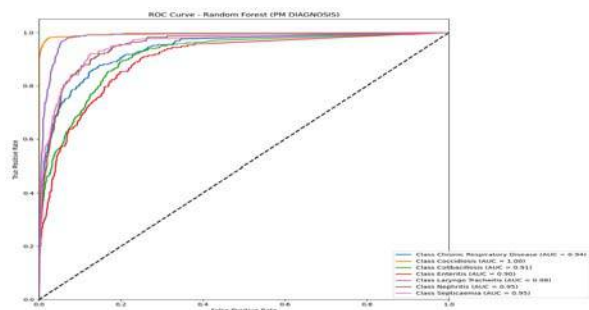
Fig. 3. ROC curve of Random Forest Classifier model
