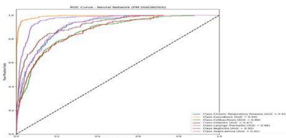
Fig. 4. ROC curve of Neural Network model
